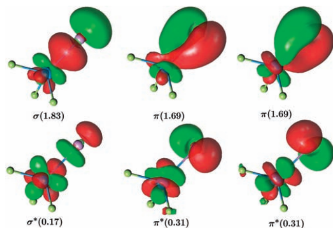
Figure 3. Active molecular orbitals in \text{As}\equiv\text{UF}_3 . Contour line 0.05 \text{ e}/\text{au}^3 . Natural orbital occupation numbers given below the orbital.
