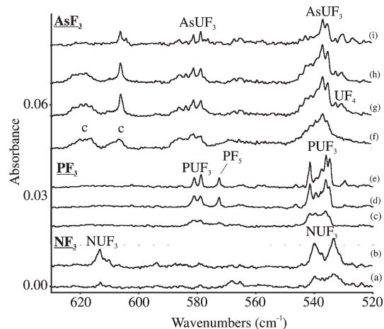
Figure 1. Infrared spectra of U atom reaction products with \text{NF}_3 , \text{PF}_3 , and \text{AsF}_3 in the 630\text{--}520\text{ cm}^{-1} region. (a) Spectrum after co-deposition of laser-ablated U and \text{NF}_3 at 0.3% in argon at 4 K for 60 min, (b) after 240\text{--}380\text{ nm} irradiation for 40 min, (c) spectrum after co-deposition of laser-ablated U and \text{PF}_3 at 0.4% in argon at 4 K for 60 min, (d) after >220\text{ nm} irradiation for 20 min, (e) after annealing to 20 K, (f) spectrum after co-deposition of laser-ablated U and \text{AsF}_3 at 0.5% in argon at 4 K for 60 min, (g) after annealing to 20 K, (h) after >220\text{ nm} irradiation for 20 min, and (i) after annealing to 30 K. Bands labeled “c” are common to \text{AsF}_3 experiments with other metals.
