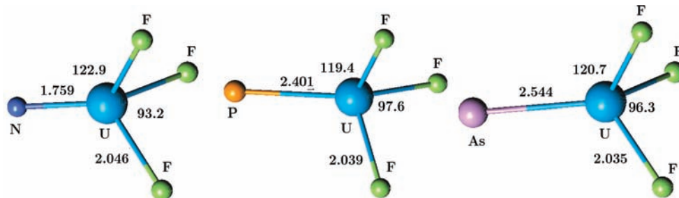
Figure 2. Structures of \text{N}\equiv\text{UF}_3 , \text{P}\equiv\text{UF}_3 , and \text{As}\equiv\text{UF}_3 in \text{C}_{3v} symmetry calculated at the CASSCF/CASPT2 level of theory. Bond lengths in angstroms and angles in degrees.
